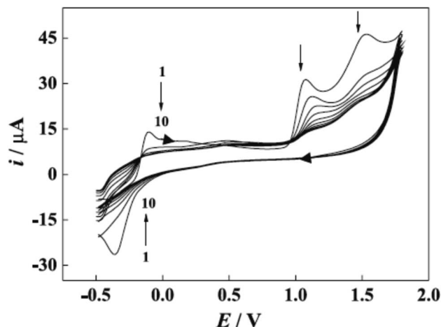
Fig. 3 CV recorded of poly(safranin) electro-polymerization in 0.1 M of sulfuric acid and scan rate: 50 mV s -1 . This figure has been adapted/reproduced from ref. 6 with permission from PubliSBQ , copyright (2023).
