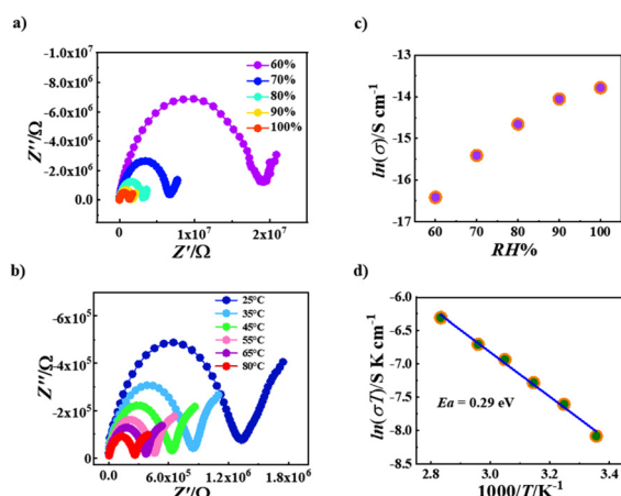
Fig. 6 Nyquist plots for R -1 at 25\text{ }^\circ\text{C} under different relative humidity (RH) levels (a). Nyquist plots for R -1 at different temperatures under 100% relative humidity (RH) (b). Plots of proton conductivity vs. RH for R -1 at 25\text{ }^\circ\text{C} (c). Plots of \ln(\sigma T) vs. 1000/T for R -1 under 100% relative humidity (RH) (d).
