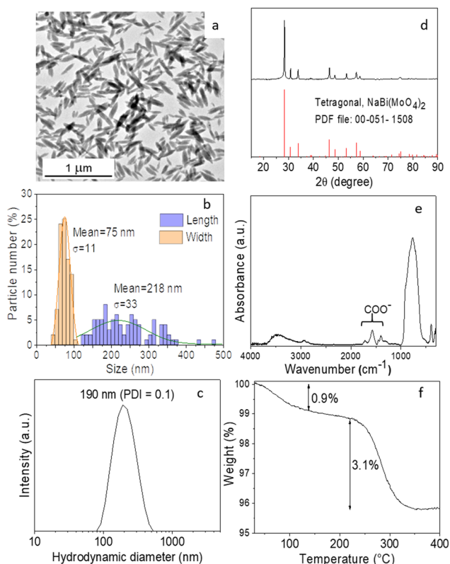
Fig. 1 (a) TEM image, (b) particle size (length and width) histogram, (c) DLS curves in Milli-Q water, (d) X-ray diffraction patterns, (e) FTIR spectrum, and (f) TGA curve of the particles synthesized by aging at 120 °C for 20 h; solutions containing 0.04 M \text{Bi}(\text{NO}_3)_3 , 0.1 M \text{Na}_2\text{MoO}_4 , and a 2 mg \text{mL}^{-1} EG/water (4/1 by vol.) mixed solvent.
