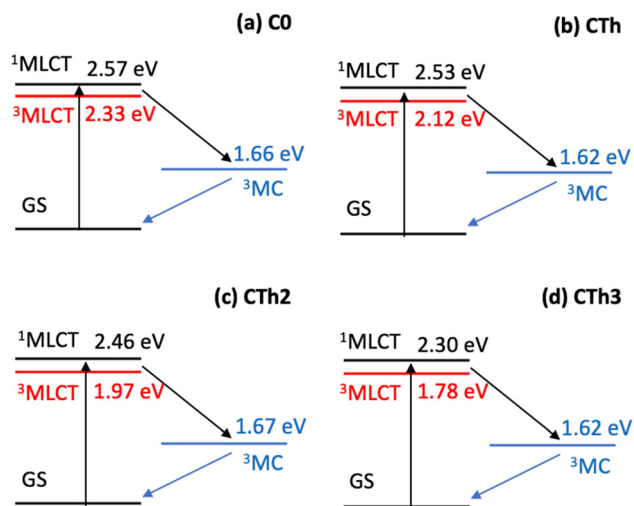
Fig. 8 Computed Jablonski diagrams of the important excited states in (a) C0 , (b) CTh , (c) CTh2 and (d) CTh3 . Using TDDFT, the energies of the ^1\text{MLCT} states were computed at the ^3\text{MLCT} optimized geometry and the energies of the ^3\text{MC} was computed at the ^3\text{MC} optimized geometry ( ^1\text{MLCT} and ^3\text{MLCT} states have similar geometries). Both geometries were computed using UKS and the relevant geometries are in the ESI.†
