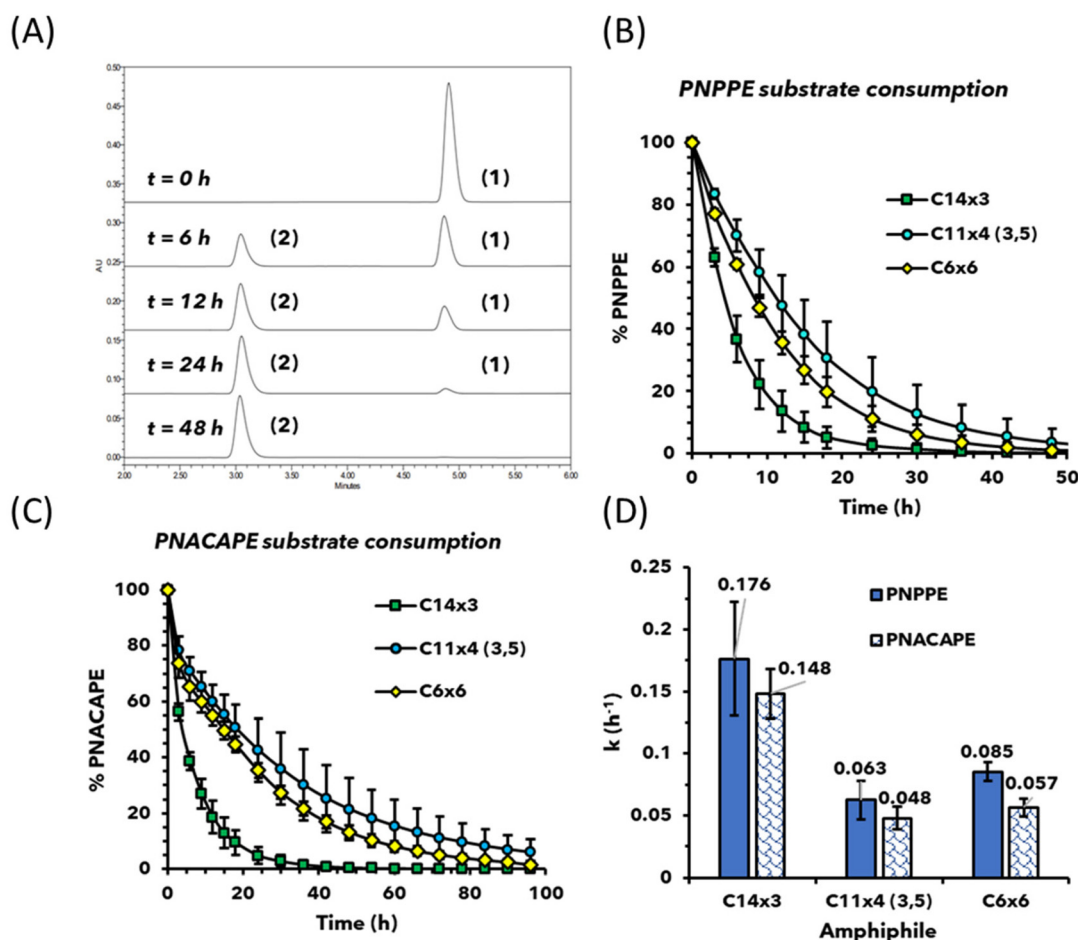
Fig. 3 (A) Representative HPLC chromatogram overlay (taken at 307 nm), showing the transformation of PNPPE (1) to para -nitrophenol (PNP) (2) using \text{Pd}^{\text{II}} loaded C14x3 amphiphilic micelles ([Amphiphile] = 320 \mu\text{M} , [PNPPE] = 300 \mu\text{M} , [ \text{Pd}(\text{OAc})_2 ] = 150 \mu\text{M} , [ \text{Pd}(\text{OAc})_2 : Substrate] = 1 : 2). Normalized substrate consumption of (B) PNPPE and (C) PNCAPE over time in the presence of C14x3 (square, green), C11x4 (3,5) (circle, deep sky blue) and C6x6 (diamond, yellow) metallic micelles. (D) Rate constants of PNPPE (blue, solid fill) and PNCAPE (blue, shingle pattern) depropargylation in presence of C14x3, C11x4 (3,5) and C6x6 metal loaded micelles.
