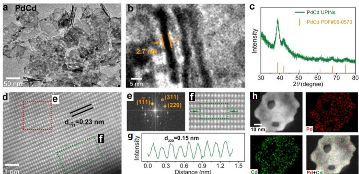
Fig. 12 Structural and compositional characterization of 2D PdCd UPINs. (a) Low-magnification TEM image. (b) HRTEM image. (c) XRD pattern. (d) Atomic-resolution aberration-corrected HAADF-STEM image. (e) FFT pattern taken from the region outlined by the red rectangle in (d). (f) Atomic-resolution HAADF-STEM taken from the region outlined by the green rectangle in (d). (g) The intensity profile taken from the region outlined by green rectangle in (d). (h) STEM-EDX elemental mapping images. This figure has been adapted from ref. 77 with permission from John Wiley and Sons, copyright 2021.
