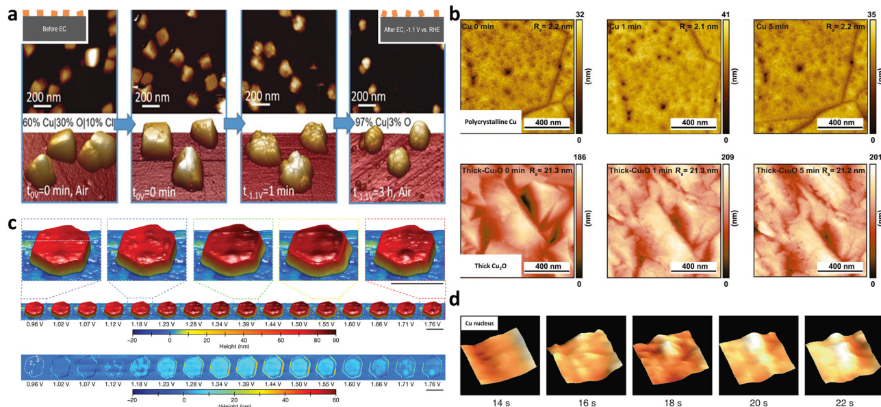
Fig. 3 (a) Dynamic morphological changes of Cu nanocubes during \text{CO}_2 RR using in situ EC-AFM in a \text{CO}_2 -saturated 0.1 M \text{KHCO}_3 aqueous solution. Cracks were observed to form on the (100) facets of Cu nanocubes, which was ascribed to the mechanical stress due to the removal of \text{Cl}^- ions (introduced by the electrodeposition of Cu cubes) from the cubes. This figure has been adapted from ref. 36 with permission from Wiley-VCH, copyright 2018. 36 (b) Monitoring surface topography or roughness over polycrystalline Cu and thick \text{Cu}_2\text{O} under \text{CO}_2 RR using quasi in situ EC-AFM in 0.1 M \text{CO}_2 -saturated \text{K}_2\text{CO}_3 electrolyte (pH 7) at -0.8 V_{\text{RHE}} . This figure has been adapted from ref. 37 with permission from NATIONAL ACADEMY OF SCIENCES, copyright 2021. 37 (c) This figure has been adapted from ref. 24 with permission from SPRINGER NATURE, copyright 2021. 24 (d) Birth and growth of a copper nucleus ( 46 \times 46 \text{ nm}^2 cropped regions) via in situ high speed LMFM. This figure has been adapted from ref. 38 with permission from SPRINGER NATURE, copyright 2017. 38
