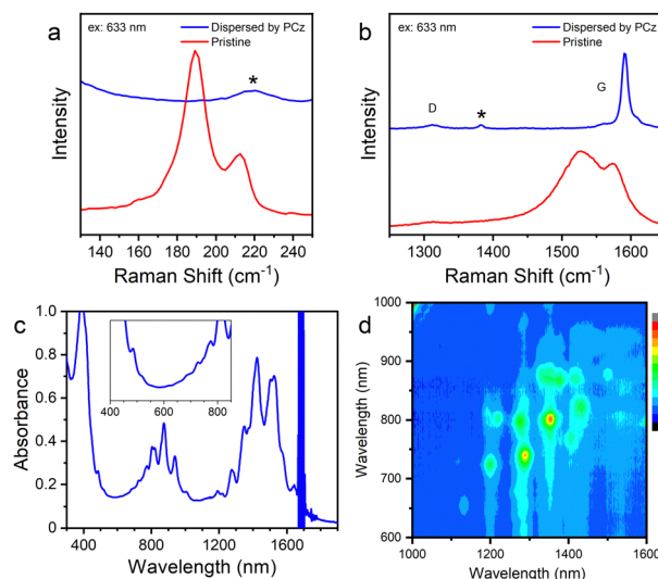
Fig. 4 Characterizations of SWCNTs dispersed by PCz in toluene. (a) and (b) Raman spectra of the SWCNT dispersion sorted by PCz in toluene (blue line) and the as-prepared SWCNTs (red line), (a) the region of RBM and (b) the region of the D-band and G-band, excitation wavelength: 633 nm, *: Raman peaks from toluene. (c) Absorption spectrum and (d) photoluminescence spectrum of the SWCNT dispersion.
