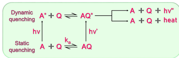
Fig. 10 Schematic diagram showing the combined mechanism of static and dynamic quenching.
