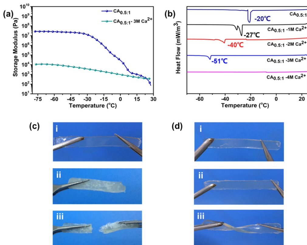
Fig. 5 Antifreezing test of ionic conductive hydrogel. (a) DMA curves of CA_{0.5:1} and CA_{0.5:1}-3\text{ M Ca}^{2+} when the temperature changes from 25 to -75\text{ }^{\circ}\text{C} , (b) DSC curves of CA_{0.5:1} and CA_{0.5:1}-\text{Ca}^{2+} when the temperature changes from 25 to -75\text{ }^{\circ}\text{C} , and (c and d) images of CA_{0.5:1} and CA_{0.5:1}-3\text{ M Ca}^{2+} bending at -50\text{ }^{\circ}\text{C} , respectively. 77
