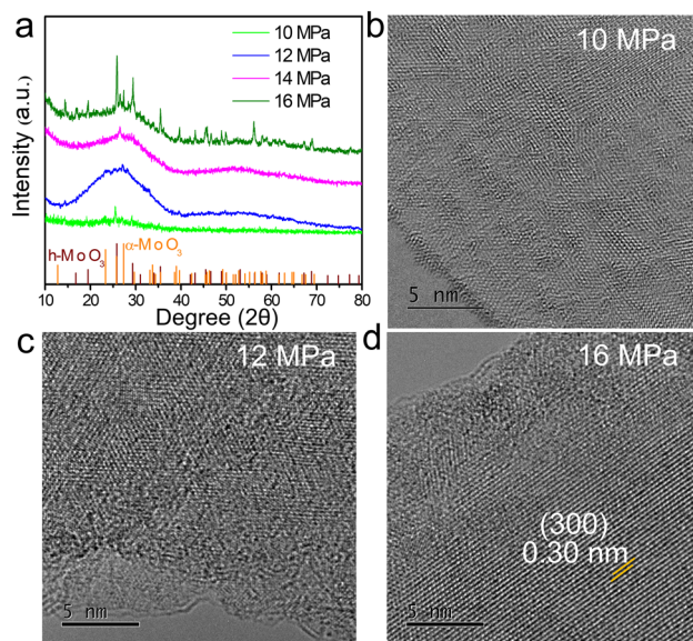
Fig. 4 (a) XRD patterns comparison of the \text{MoO}_{3-x} obtained at different pressures, and XRD patterns at the bottom show \alpha\text{-MoO}_3 (JCPDS No. 05-0508) and \text{h-MoO}_3 (JCPDS No. 21-0569); (b–d) HRTEM images of the \text{MoO}_{3-x} sample obtained at 10 MPa, 12 MPa, 16 MPa.
