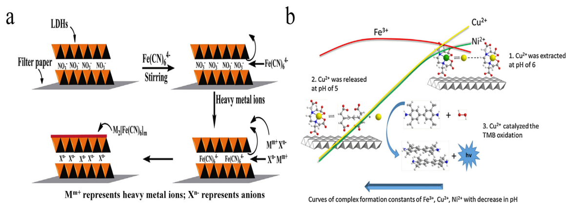
Fig. 2 (a) Illustration of the concept for the formation of Fe(CN) 6 4- anion-interlayered MgAl-LDH-modified test strips and the detection of heavy metal ions. Reprinted with permission from ref. 44. Copyright 2016, Elsevier. (b) Schematic of the selective extraction–release–catalysis detection process. Reprinted with permission from ref. 45. Copyright 2015, Elsevier.
