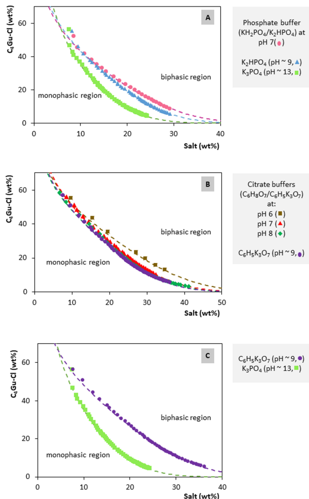
Fig. 2 Binodal curves of the ABSs composed of C_4Gu-Cl IL + salt + H_2O at 25\text{ }^\circ\text{C} : (A) effect of the salt anion in the ABS formation ability using phosphate salts, (B) effect of the pH in the ABS formation ability using citrate salts, (C) effect of the salt nature in the ABS formation ability using phosphate versus citrate salts. Dashed lines represent the adjusted binodal data using eqn (1) (–).
