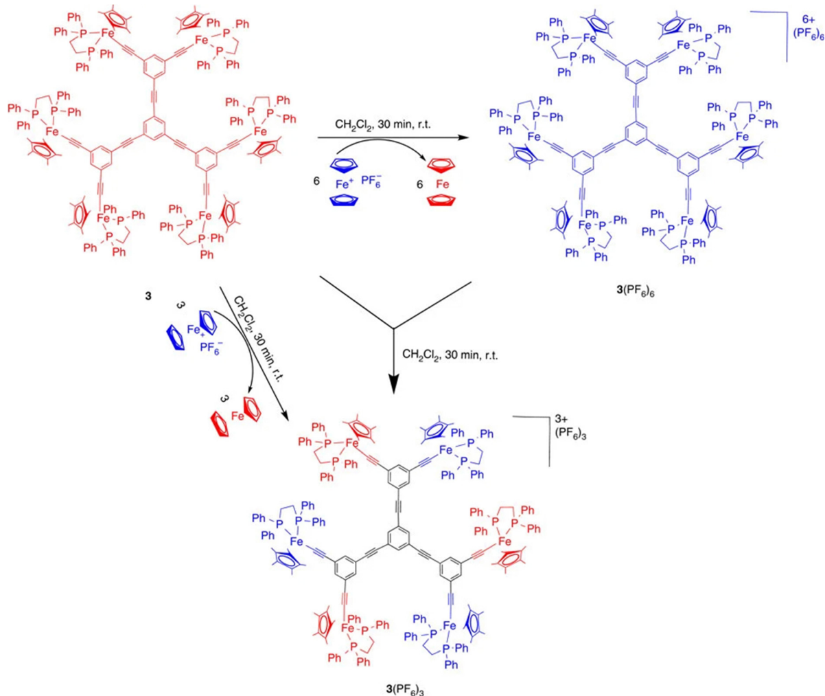
Scheme 9 Syntheses using the 17-electron ferricenium complex of both the \text{Fe(III)} and class-II mixed-valent \text{Fe(II)-Fe(III)} hexanuclear complexes. The latter can also be obtained by quantitative comproportionation between the \text{Fe(II)} and \text{Fe(III)} hexanuclear complexes. Various dendrimers containing the same mixed-valent \text{Fe(II)-Fe(III)} periphery were obtained in the same way (see Fig. 6). Blue represents \text{Fe(II)} , and red, \text{Fe(III)} . Reproduced with permission from ref.76 Copyright 2014 Springer Nature.
