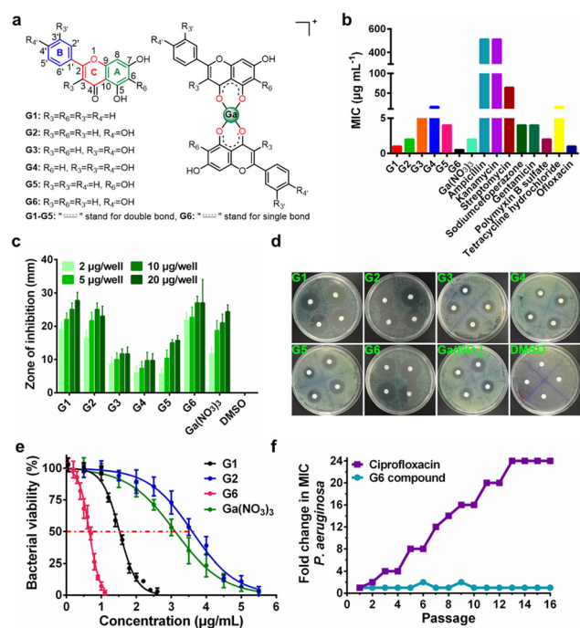
Fig. 1 Anti-bacterial activity of gallium-flavonoid compounds in vitro . (a) The chemical structures of flavonoid ligands and gallium compounds. (b) The minimum inhibitory concentration (MIC) of gallium-flavonoid compounds and antibiotics against P. aeruginosa . (c) Diameters of inhibition zones of gallium compounds, \text{Ga}(\text{NO}_3)_3 , and DMSO. (d) Representative figures of the agar diffusion test. (e) Bacterial viability assay for gallium-flavonoid compounds and \text{Ga}(\text{NO}_3)_3 . The \text{IC}_{50} values of G1 , G2 , G6 and \text{Ga}(\text{NO}_3)_3 are 1.52, 3.59, 0.65, and 3.11 \mu\text{g mL}^{-1} , respectively. All experiments are performed in triplicates, and data are presented as mean \pm SD. (f) Resistance development of P. aeruginosa PAO1 toward G6 and ciprofloxacin. Values are fold changes in minimal inhibitory concentration (MIC) relative to the MIC of the first passage.
