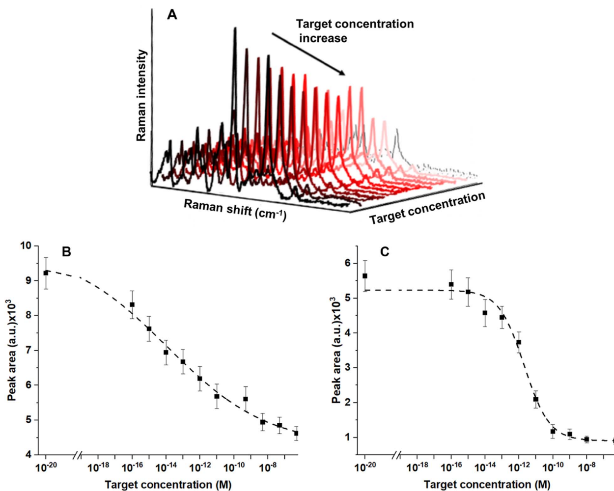
Fig. 6 SERS spectra of the MB-decorated biosensor as a function of T concentration (A); plot of ROX peak area at 1646 \text{ cm}^{-1} as a function of T concentration for the MB biosensor (B) and MB-MCH biosensor (C).
