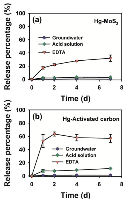
Fig. 5 Desorption kinetics of Hg from (a) \text{MoS}_2 and (b) activated carbon in the groundwater, acid solution, and EDTA solution, initial C_{\text{Hg}} = 20 \text{ mg L}^{-1} , C_{\text{MoS}_2} = 8 \text{ mg L}^{-1} , C_{\text{AC}} = 1.67 \text{ g L}^{-1} .
