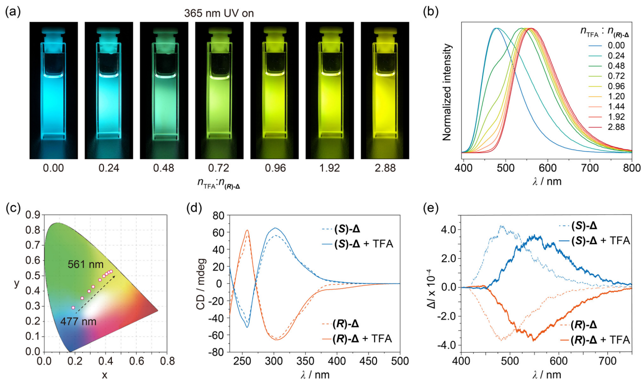
Fig. 3 Photophysical properties of ( R - and ( S - \Delta . (a) Luminescence photographs taken upon shining 365 nm UV light. (b) Fluorescence spectra upon excitation at 380 nm. (c) Trajectory of tuning colors shown in the CIE coordinate diagram of solutions ( 1 \times 10^{-5} M) of ( R - \Delta in \text{CHCl}_3 containing different amounts of TFA relative to ( R - \Delta ranging from 0 to 2.88 equiv. (d) CD and (e) CPL spectra of solutions ( 2 \times 10^{-4} M) of ( R - and ( S - \Delta in deacidified \text{CHCl}_3 (dash line) and in acidified \text{CHCl}_3 with TFA ( 2.88 \times 10^{-5} M, solid line).
