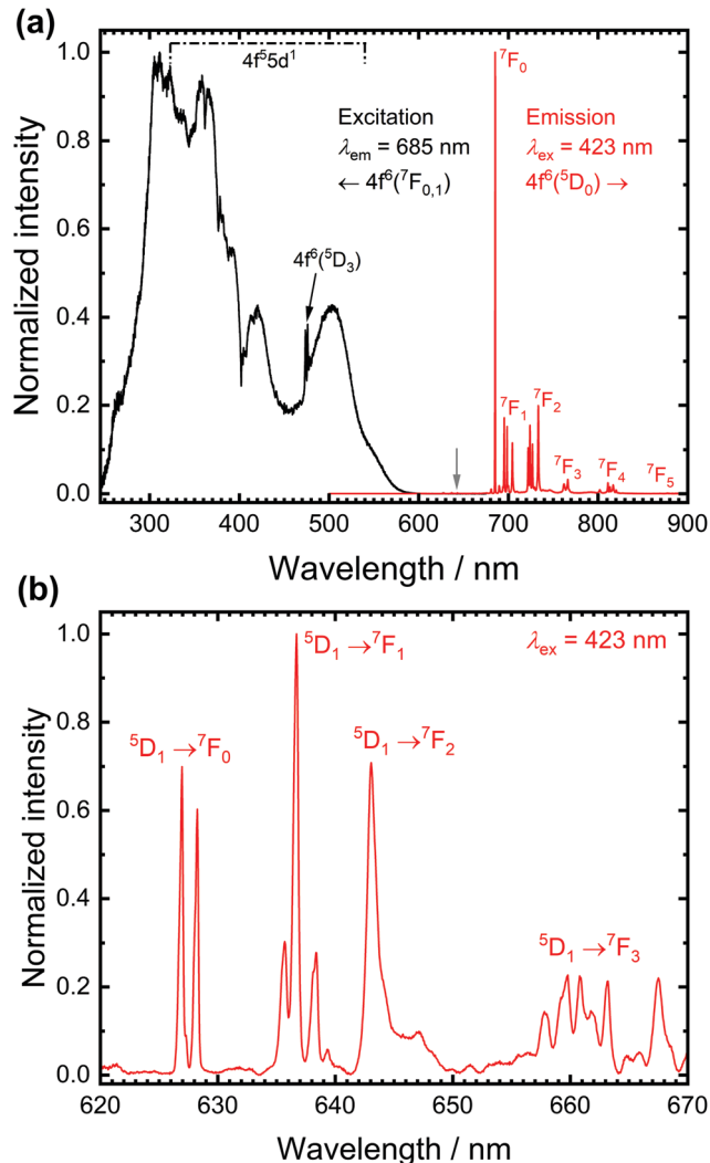
Fig. 1 (a) Photoluminescence excitation (black, \lambda_{\text{em}} = 685 \text{ nm} ) and emission (red, \lambda_{\text{ex}} = 423 \text{ nm} ) spectrum of \text{SrB}_4\text{O}_7:0.5\% \text{Sm}^{2+} at room temperature. The emission lines are assigned to the {}^5\text{D}_0 \rightarrow {}^7\text{F}_J ( J = 0 \dots 6 ) transitions of \text{Sm}^{2+} . (b) High-resolution spectrum in the spectral range marked with the grey arrow in (a) indicates the presence of weak {}^5\text{D}_1 \rightarrow {}^7\text{F}_J transitions.
