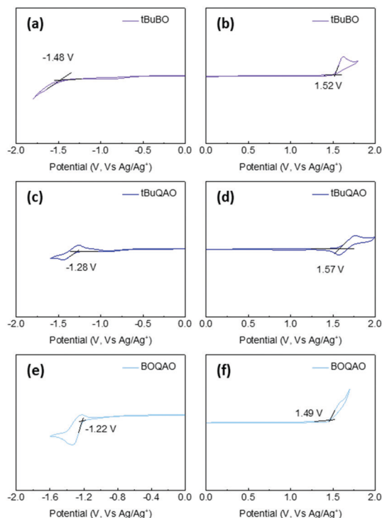
Fig. 2 Cyclic voltammety (CV) curves of (a and b) t BuBO, (c and d) t BuQAO, and (e and f) BOQAO .
