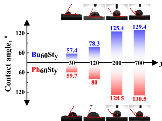
Fig. 3 The contact angle (CA) of \text{Bu}_{60}\text{Sty}_x\text{-M} and \text{Ph}_{60}\text{Sty}_x\text{-M} in membrane form. The \text{Bu}_{60} and \text{Ph}_{60} macro-CTAs were soluble in water.
