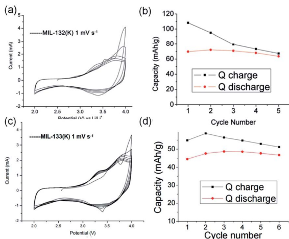
Fig. 21 (a) The solid-state cyclic voltammetry of MIL-132(K) between the 2 and 4 V vs. Li/Li + at 1 mV s -1 ; (b) the charge and discharge capacity of MIL-132(K) within 5 cycles; (c) the solid-state cyclic voltammetry of MIL-133(K) between the 2 and 4 V vs. Li/Li + at 1 mV s -1 ; (d) the charge and discharge capacity of MIL-133(K) within 6 cycles. Reprinted with permission from ref. 44. Copyright 2010, American Chemical Society.
