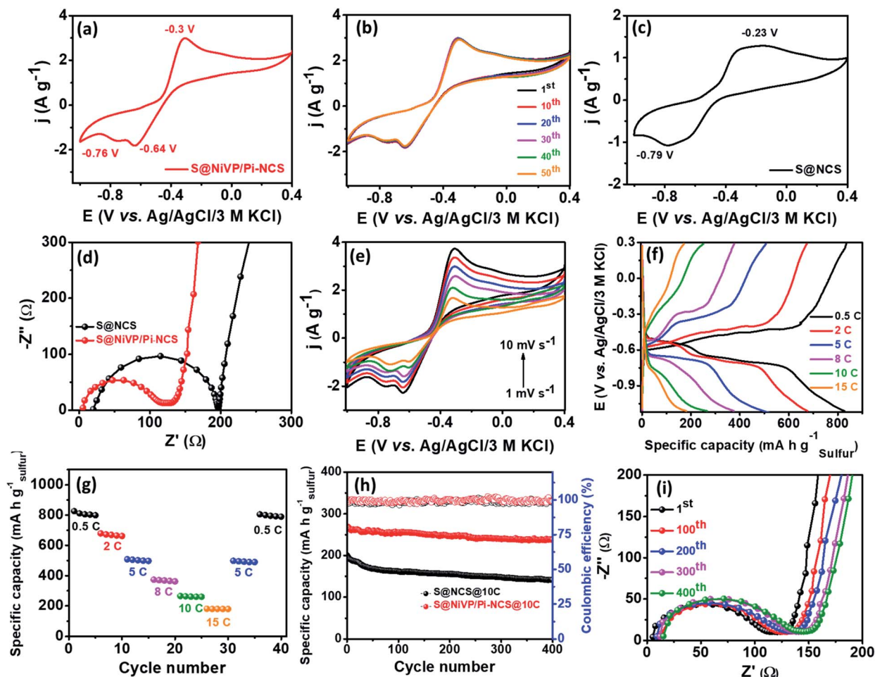
Fig. 3 (a) CV and (b) cyclic stability of S@NiVP/Pi-NCS for 50 cycles at 2 mV s -1 ; (c) CV of S@NCS anode at 2 mV s -1 ; (d) EIS spectra of the respective anodes; (e) CVs at various scan rates; (f) voltage profile of S@NiVP/Pi-NCS; (g) rate performance of S@NiVP/Pi-NCS anode at different C-rates; (h) long term cycling performance of various anodes at 10C over 400 cycles in 2 M aq. Na 2 SO 4 and (i) the corresponding EIS during cycling performance.
