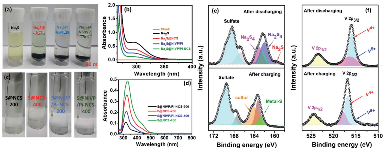
Fig. 4 (a) Photographic images of the Na 2 S solution with various catalysts after 30 minutes, (b) corresponding UV-vis spectra of Na 2 S solution of Fig. 4a after 30 minutes, (c) photographic images of 2 M aq. Na 2 SO 4 electrolyte with S@NiVP/Pi-NCS and S@NCS anodes after 200 and 400 cycles, and (d) corresponding UV-vis spectra of dissolved polysulfide in 2 M aq. Na 2 SO 4 at various cycling performances, deconvoluted XPS spectra of (e) S 2p and (f) V 2p of S@NiVP/Pi-NCS anode after the charge and discharge cycles.
