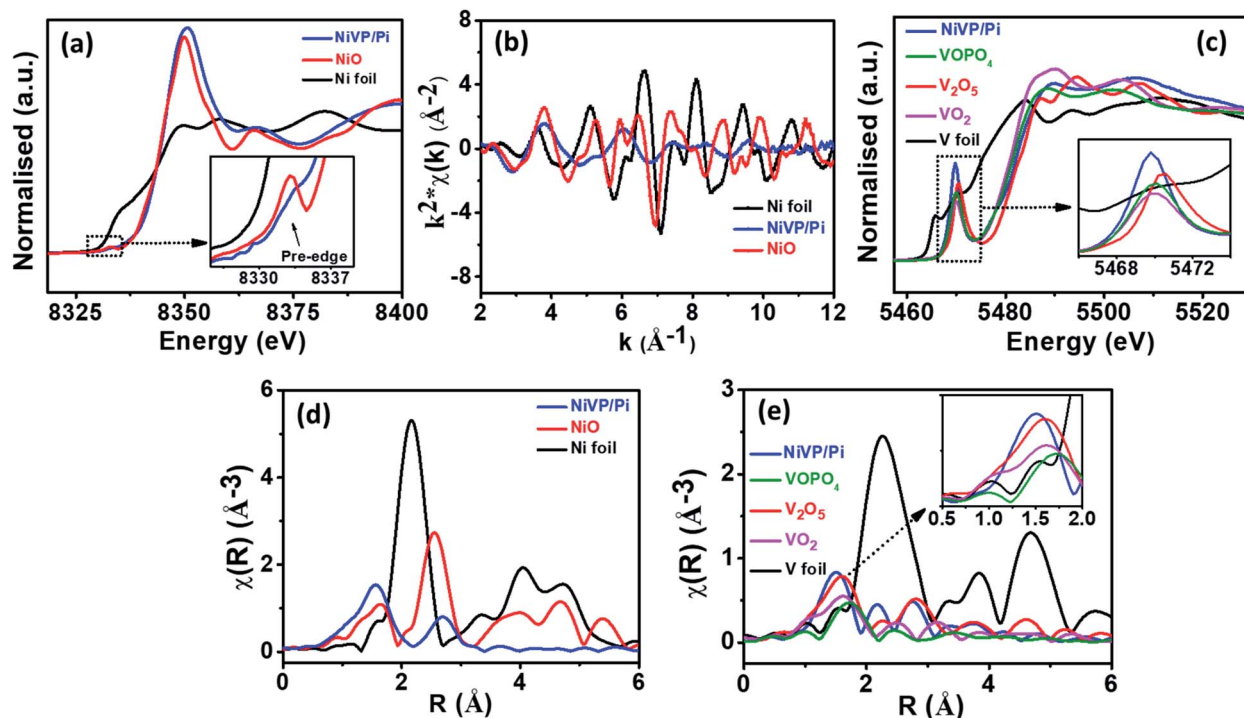
Fig. 2 (a) Normalized XANES spectra of NiVPi/Pi along with standard samples at the Ni K-edge, (b) EXAFS oscillation of NiVPi/Pi along with standard samples in k -space at the Ni K-edge, (c) XANES spectra of NiVPi/Pi and Fourier transform EXAFS spectrum at (d) Ni K-edge and (e) V K-edge of NiVPi/Pi along with the standards.
