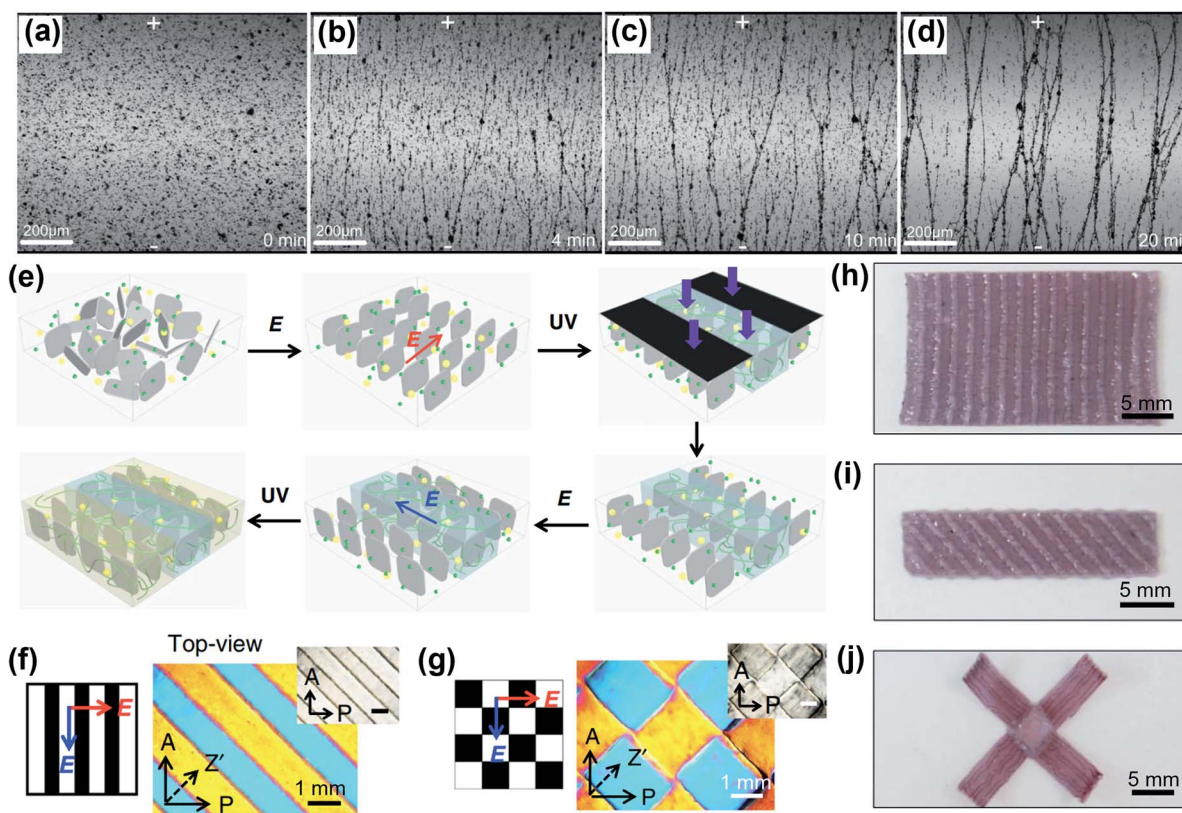
Fig. 16 Controlled orientation induced by an electric field. (a–d) Optical micrograph images of graphene nanoplatelet alignment in liquid epoxy resin by an AC electric field ( E ) as a function of time (0 to 20 min). (a) Random orientation of graphene nanoplatelets before applying an electric field, and after applying an electric field for (b) 4 min, (c) 10 min and (d) 20 min. Reproduced from ref. 233 with permission from Elsevier. (e) Schematic representation of a patterned anisotropic hydrogel by multi-step electrical orientation and photolithographic polymerization with different electric field ( E ) directions and use of ultraviolet (UV) light. (f and g) Polarizing optical microscope (POM) images showing hydrogel patterns with different nanosheet alignments. A: analyzer, P: polarizer, and Z': axis of the tint plate. (h–j) Photos of the patterned anisotropic hydrogels. Reproduced from ref. 232 with permission from Springer Nature.
