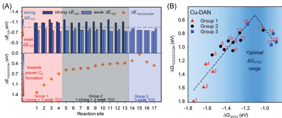
Fig. 2 (A) Individual \ast CO adsorption energies 6 (upper panel) and corresponding \ast CO-CO-COH formation energies (lower panel) on 17 reaction sites on Cu-DANs. These 17 reaction sites are classified into three groups according to the individual \ast CO adsorption strength. The blue dashed line in the upper panel indicates the benchmark between strong and weak \ast CO adsorption ( -0.87 V). 53 Detailed atomic structures, and \ast CO and \ast CO-CO-COH adsorption configurations can be found in Table S3 and Fig. S2–S18.† (B) Activity volcano plot between \ast CO adsorption free energy ( \Delta G_{\ast CO} ) and corresponding \ast CO-CO-COH formation free energy ( \Delta G_{\ast CO-CO-COH} ) on the 17 reaction sites (numbered in red) of Cu-DAN. The optimal range for \ast CO adsorption toward \ast CO-CO-COH formation is highlighted in dark blue.
