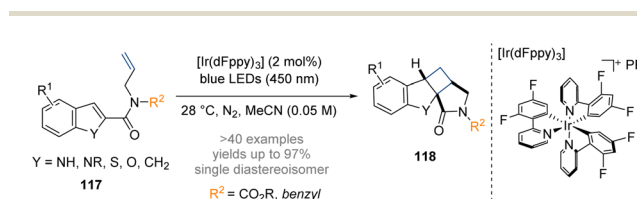
Scheme 34 Dearomative photoredox catalysed intramolecular [2 + 2] cycloaddition of indoles. 40
