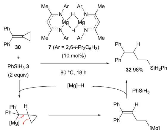
Scheme 8 1,2-Dimagnesiobutene 30 with Mg(I) dimer 20 followed by \beta -alkyl migration and its catalytic variant with Mg(II) hydride 7 (Crimmin, 2020).
