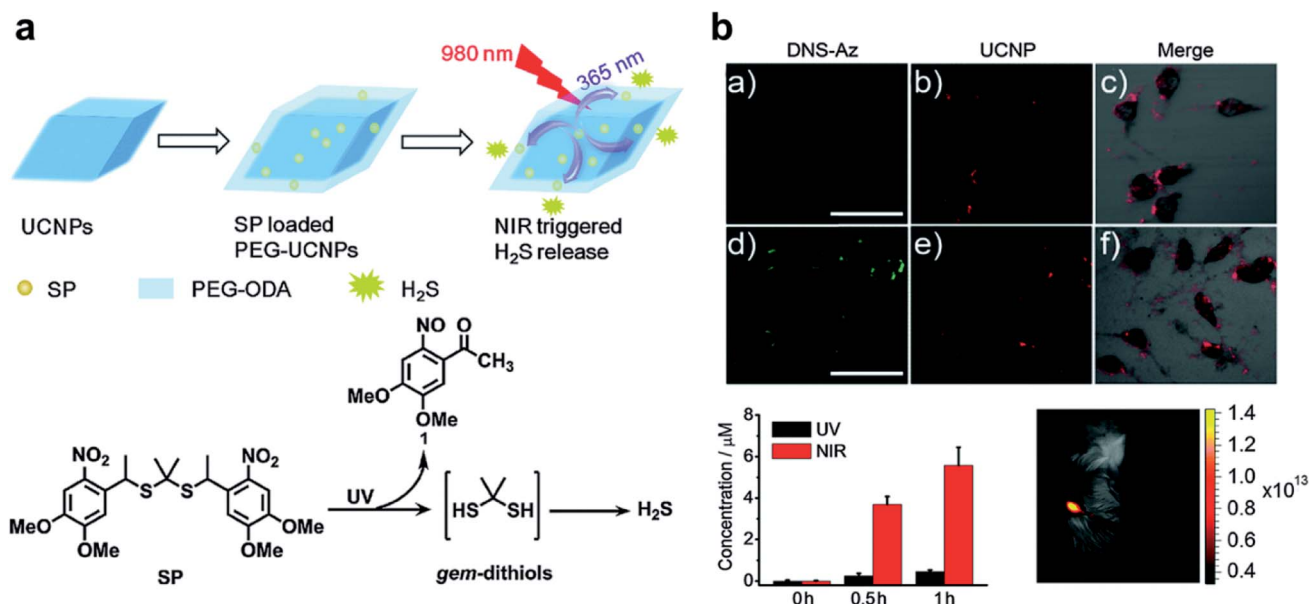
Fig. 6 UCNP-based nanocomposites for H 2 S gas therapy. (a) Construction of SP-loaded PEG-UCNP platform for NIR-triggered H 2 S release. (b) H 2 S release from SP-loaded PEG-UCNPs with laser irradiation. 38 Adapted from ref. 38 with permission from Royal Society of Chemistry, copyright 2015.
