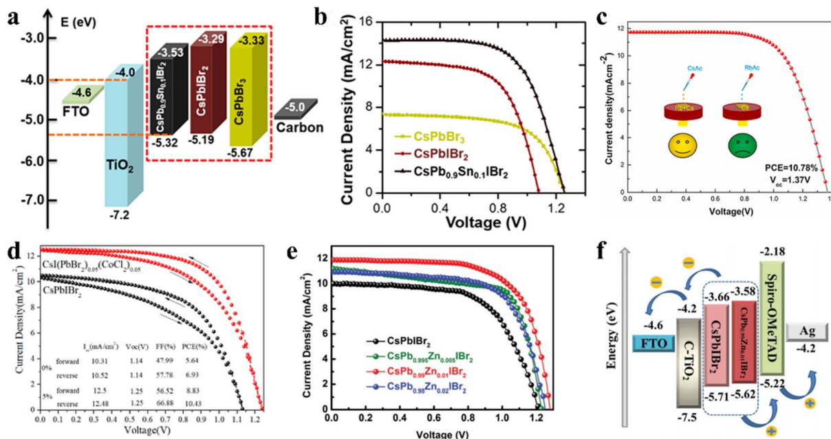
Fig. 10 (a). Energy level diagrams of IPSCs. (b). J - V plots of IPSCs based on \text{CsPbBr}_3 , \text{CsPbIBr}_2 , and \text{CsPb}_{0.9}\text{Sn}_{0.1}\text{IBr}_2 , respectively. (a and b) Reprinted with permission. 110 Copyright 2017, the American Chemical Society. (c). J - V curves of IPSCs with multi-source Rb/Ac-doped \text{CsPbIBr}_2 films. Reproduced with permission. 114 Copyright 2021, Elsevier. (d). J - V curves of optimal \text{CsPbIBr}_2 and \text{CsI}(\text{PbBr}_2)_{1-x}(\text{CoCl}_2)_x devices under forward and reverse scans. Reproduced with permission. 115 Copyright 2020, Elsevier. (e). J - V curves of the \text{CsPb}_{1-x}\text{Zn}_x\text{IBr}_2 ( x = 0, 0.005, 0.01 and 0.02 ) IPSCs under simulated AM1.5G illumination. (f). Corresponding energy level diagrams with \text{CsPbIBr}_2 and \text{CsPb}_{0.99}\text{Zn}_{0.01}\text{IBr}_2 devices. (e and f) Reproduced with permission. 117 Copyright 2021, The Royal Society of Chemistry.
