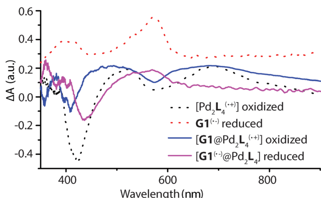
Fig. 6 Electrochemically generated difference absorption spectra for the oxidized [\text{Pd}_2\text{L}_4]^{4+} , [\text{G1@Pd}_2\text{L}_4]^{4+} and reduced \text{G1}^{(--)} , [\text{G1}^{(--)@Pd}_2\text{L}_4] species (number of oxidized L units and overall charges not specified in formulas). UV-Vis spectra of samples recorded during cyclic voltammetry with a scan rate of 0.1\text{ V s}^{-1} , Pt gauze as working electrode and \text{Ag}/\text{AgNO}_3 as reference electrode.
