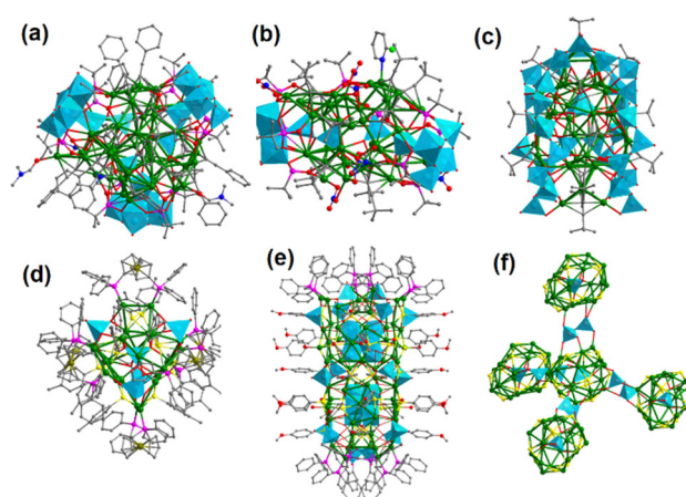
Fig. 18 Molecular structures of (a) [(\text{O}_2)\text{V}_2\text{O}_6]_3@[\text{Ag}_{43}@[(^t\text{BuPO}_3)_4\text{V}_4\text{O}_8]_3] , (b) [(\text{O}_2)\text{V}_2\text{O}_6]_2@[\text{Ag}_{36}@[(^t\text{BuPO}_3)_4\text{V}_4\text{O}_8]_2] , (c) (\text{V}_2\text{O}_7)_2@[\text{Ag}_{44}(\text{V}_{32}\text{O}_{96})] , (d) \text{MoO}_4@[\text{Ag}_{24}@(\text{MoO}_4)_4] and (e) (\text{MoO}_4)_5@[\text{Ag}_{52}@(\text{MoO}_4)_{10}] . (f) Each \text{CrO}_4@[\text{Ag}_{20} \text{ subunit connected to its adjacent four neighbours by } \text{Cr}_2\text{O}_7^{2-}] . (g) Molecular structure (left) and cyclic voltammogram (right) of \text{SiW}_{10}\text{O}_{37}@[\text{Ag}_{41}-\beta\text{-SiW}_{12}\text{O}_{40}] .
