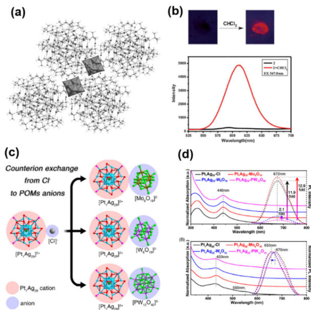
Fig. 17 (a) Packing diagram and (b) luminescence change induced by \text{CHCl}_3 of [\text{Ag}_{62}\text{S}_{13}(\text{S}^t\text{Bu})_{32}][\text{Mo}_6\text{O}_{19}]_2 . Reproduced with permission from ref. 62. Copyright 2012, Wiley-VCH. (c) Structures and the optical absorptions and (d) emissions of \text{Pt}_1\text{Ag}_{28}-\text{Mo}_6\text{O}_{19} , \text{Pt}_1\text{Ag}_{28}-\text{W}_6\text{O}_{19} and \text{Pt}_1\text{Ag}_{28}-\text{PW}_{12}\text{O}_{40} . Reproduced with permission from ref. 63. Copyright 2021, American Chemical Society.
