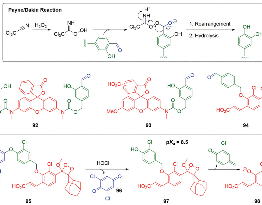
Scheme 19 Yang and Shabat's sensors for oxidative activity the cell triggered by H_2O_2 or HOCl . 137–139
