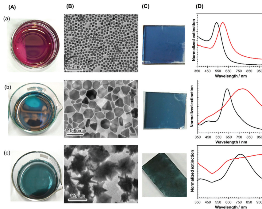
Fig. 2 Assembly of various metal nanocrystals by using the developed methodology: (a) Au nanospheres with a diameter of 16 \pm 2 nm, (b) AgPRs with an edge length of 59 \pm 7 nm, and (c) Au nanostars with a size of 93 \pm 12 nm. These assembled films were prepared at the air–water interface by dropping a BuOH dispersion (400 \mu L) into the water phase (8000 \mu L) and leaving it for 2 h. (A) Photographs of the films at the air–water interface, (B) TEM images, (C) photographs of films transferred onto glass substrates, and (D) extinction spectra of the BuOH dispersion (black lines) and the transferred films (red lines).
