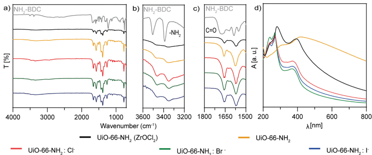
Fig. 4 (a–c) FTIR analysis and (d) UV-vis spectroscopy of UiO-66-NH 2 NMOFs: UiO-66-NH 2 (ZrOCl 2 ) (black), UiO-66-NH 2 (orange), UiO-66-NH 2 :Cl − (red), UiO-66-NH 2 :Br − (green) and UiO-66-NH 2 :I − (blue).
