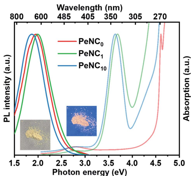
Fig. 3 UV-Vis absorption and PL spectra of \text{PeNC}_0 ( \lambda_{\text{ex}} = 275 \text{ nm} ), \text{PeNC}_1 ( \lambda_{\text{ex}} = 330 \text{ nm} ), and \text{PeNC}_{10} ( \lambda_{\text{ex}} = 330 \text{ nm} ) with nanocrystals in the powder form. Photographs showing the \text{PeNC}_1 powder sample under room illumination (left) and UV irradiation (right).
