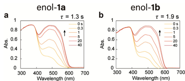
Fig. 2 Ultraviolet-visible diffuse reflectance spectra of powder (a) enol- 1a and (b) enol- 1b crystals upon irradiation with a UV light-emitting diode (LED).
