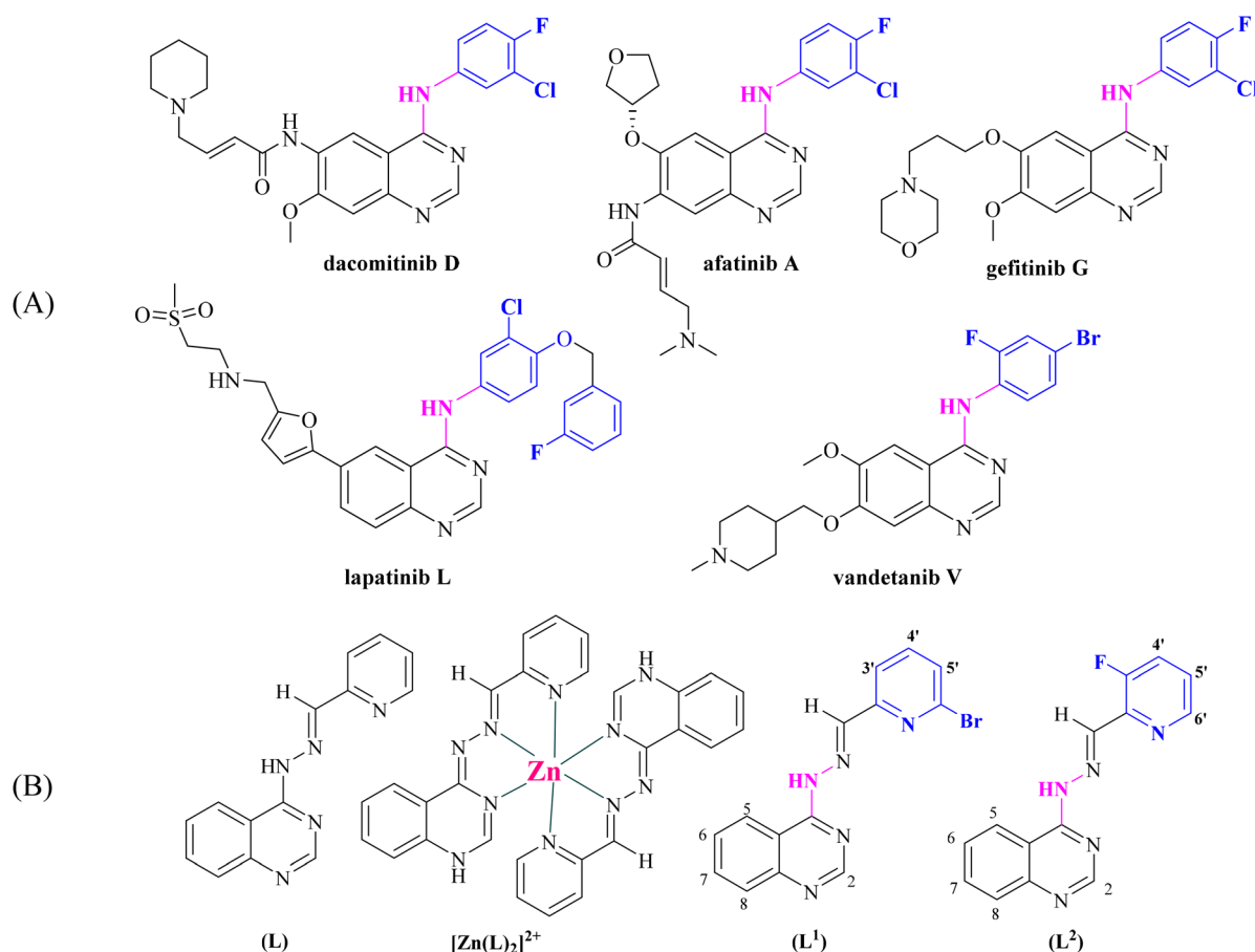
Fig. 1 (A) Quinazoline derivatives approved by the FDA as anticancer agents. (B) Ligand ( L ) used in our previous studies 25–27 and its Zn complex [Zn(L) 2 ] 2+ . 27 Evolution of the structure of [( E )-4-(2-(pyridin-2-ylmethylene)hydrazinyl)quinazoline] ( L ) into possible halogenated pharmacophores [( E )-4-(2-((6-bromopyridin-2-yl)methylene)hydrazinyl)quinazoline] ( L 1 ) and [( E )-4-(2-((3-fluoropyridin-2-yl)methylene)hydrazinyl)quinazoline] ( L 2 ) (aromatic H atoms numbering is also shown).
