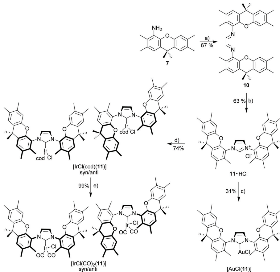
Scheme 4 Synthesis of imidazolium salt 11 ·HCl and derived metal complexes. Reagents and conditions: (a) glyoxal, p TsOH, EtOH, 50 °C; (b) paraformaldehyde, Me 3 SiCl, EtOAc, 70 °C, 24 h; (c) [AuCl(SMe 2 )], K 2 CO 3 , acetone, 50 °C; (d) [IrCl(cod)] 2 , K 2 CO 3 , acetone, 50 °C; (e) CO, 0 °C, 30 min, CH 2 Cl 2 .
