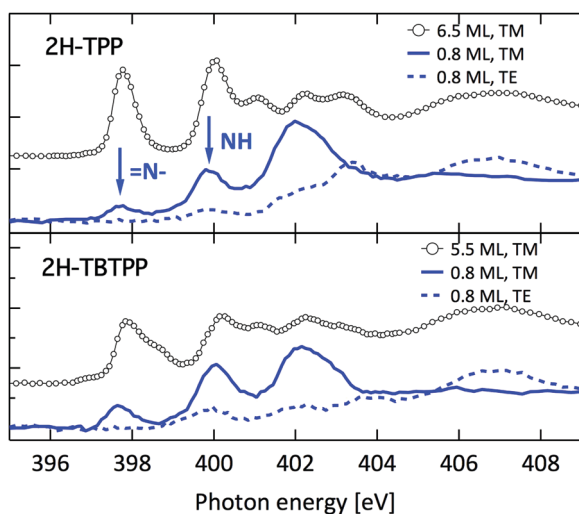
Fig. 6 Nitrogen K-edge NEXAFS spectra of the 2H-TPP and 2H-TBTP films of Fig. 3 (top and bottom panels, respectively). NEXAFS measurements in TM and TE polarization (full and dashed lines, respectively) are shown for the 0.8 ML films, whereas only spectra in TM polarization are shown for multilayers (open markers).
