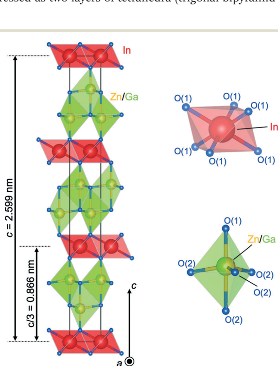
Fig. 5 Crystal structure of \text{InGaO}_3(\text{ZnO})_1 . Coordination of \text{InO}_6 is octahedra and \text{Zn/GaO}_5 is trigonal bipyramid. Because Zn and Ga cannot be separated, the Zn/Ga mixed site is referred to as the trigonal bipyramid in this paper.
