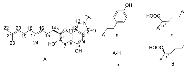
Scheme 1 Molecular structures of Stachybotrin C and selected SMTP, (a) Stachybotrin C, (b) SMTP-0, (c) SMTP-7, and (d) SMTP-7D. The stereocenters in investigation are labeled with stars.
