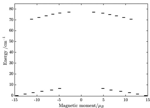
Fig. 12 Calculated low-lying spin–orbit manifolds of states arising from the magnetic interaction between the ground multiplet S = 5/2 of the Fe III ion and the ground and first excited Kramers doublet of the Dy III ion. The components of each doublet (black lines) are placed on the diagram according to their magnetic moment projection on the main magnetic axis of the ground doublet (with energy zero).
