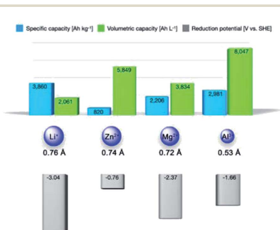
Fig. 1 Specific capacities, volumetric capacities, ionic radii, and stripping/plating potentials of various metal ions.
