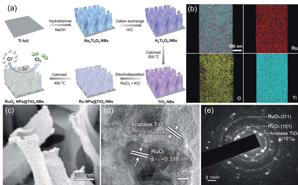
Fig. 10 (a) Schematic diagram of the \text{RuO}_2 NPs@ \text{TiO}_2 NB synthesis process. (b) Energy-dispersive X-ray spectroscopy (EDX) images of \text{RuO}_2 NPs@ \text{TiO}_2 NBs. (c) SEM images of \text{RuO}_2 NPs@ \text{TiO}_2 NBs. (d) TEM images and (e) SAED analysis of \text{RuO}_2 NPs@ \text{TiO}_2 NBs. Reproduced with permission. 48 Copyright 2020, Elsevier.
