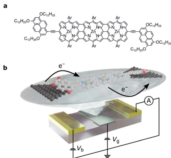
Fig. 1 (a) The molecular structure of FP3 : the edge-fused porphyrin trimer core is functionalized in the terminal meso positions by tridodecylloxy groups for anchoring to graphene source and drain electrodes. Ar groups are solubilizing aryl groups, 3,5-bis(trihexylsilyl) phenyl. (b) Device architecture: nanometer-separated graphene source and drain electrodes are electroburnt from a graphene ribbon between two gold electrodes. The graphene is patterned into a bowtie shape, and a local gate electrode separated from the molecule by a thin layer of \text{HfO}_2 (grey) is used to shift the molecular energy levels. For clarity, the bulky side-groups are omitted.
