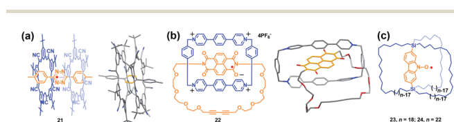
Fig. 9 (a) Stabilizing the tetrazine radical anion using size-matched, anion-binding cyanostar macrocycles (21). Reproduced from ref. 36a. (b) Stabilizing the naphthalenediimide radical within a tetracationic cyclophane (22). Reproduced from ref. 36b. (c) Structures of the macrocages with a bridged carbazole nitroxide (23 and 24). Reproduced from ref. 39.
