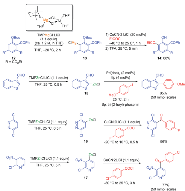
Scheme 5 Directed magnesiations and zincations using mixed Mg–Li or Zn–Li–TMP-bases.
