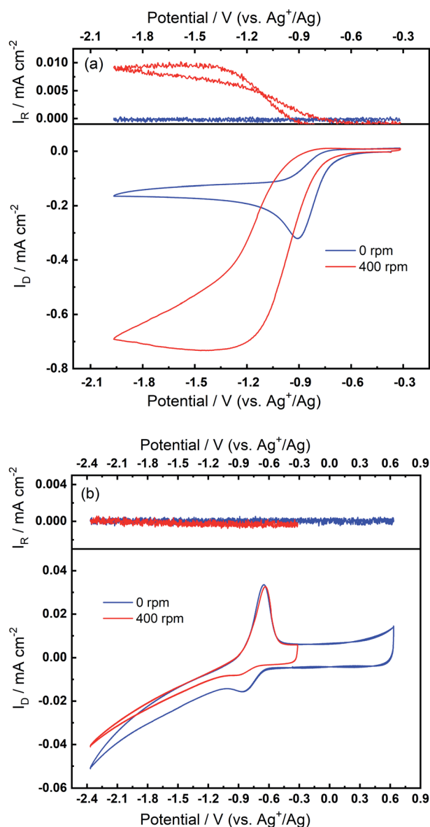
Fig. 7 RRDE measurements at 100 \text{ mV s}^{-1} with rotation speeds of 0 rpm and 400 rpm (a) before and (b) after the oxidation peak appears in \text{O}_2 -bubbled 0.1 \text{ M TBAClO}_4/0.01 \text{ M Ca(ClO}_4)_2/\text{DMSO} . The disc and ring electrodes are GC and Pt, respectively, and the potential of ring is -0.37 \text{ V} . A potential limit of -2.37 \text{ V} is set in (b), in accordance with previous CVs wherein the reversible OER peak can be found.
