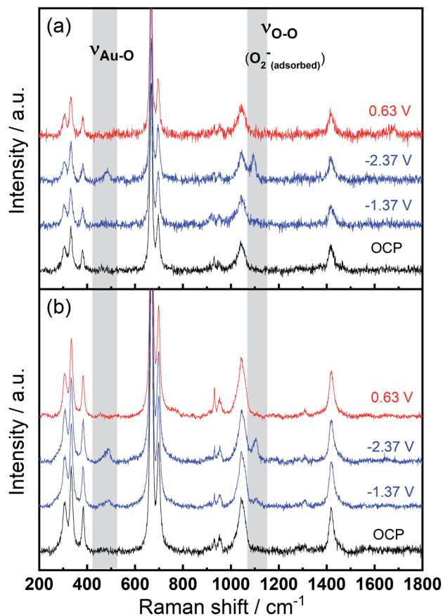
Fig. 6 In situ SERS (normalised) measured at various potentials on a roughened Au electrode in \text{O}_2 -saturated (a) 0.1 \text{ M TBAClO}_4/0.01 \text{ M Ca(ClO}_4)_2/\text{DMSO} and (b) 0.1 \text{ M TBAClO}_4/\text{DMSO} .
