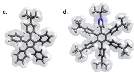
Fig. 1 Selection of pioneering examples of molecular cogwheel systems exhibiting intramolecular gearing in solution (a and b) or intermolecular gearing when anchored on a surface (c and d). These selected examples have been reported by (a) Iwamura, 20 (b) Siegel, 21 (c) Moresco 22 and (d) Soe. 23
