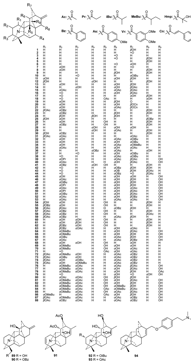
Fig. 2 The amine subtype alkaloids (1–94) of hetisine (the names of the alkaloids are given in ESI Table S1†).
